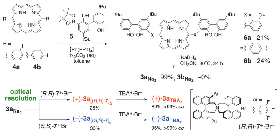
Scheme 1. Synthesis of the boron helicate 3a Na 2 and its optical resolution by the formation of a diastereomeric salt with optically pure ( R,R )- or ( S,S )- 7 . The chiral ammonium ( 7 ) was then replaced with the achiral ammonium salt TBA + .Br − .
